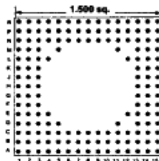
153 PINS Footprint 15017
