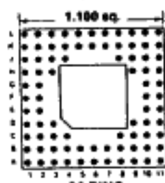
Footprint 11011
