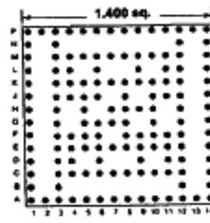
139 PINS Footprint 14010
