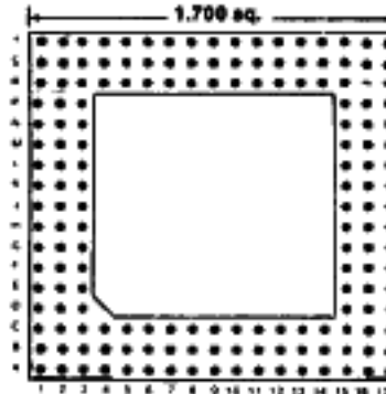
168 PINS Footprint 17009
