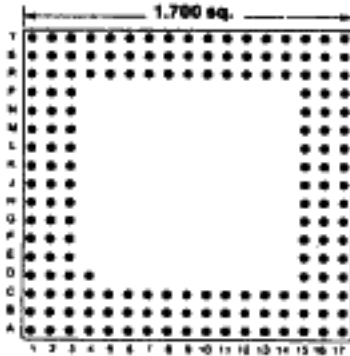
169 PINS Footprint 17012
