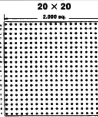
400 PINS Footprint 20001
