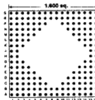
172 PINS Footprint 16002
