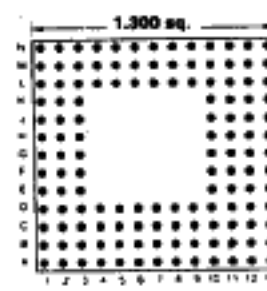
133 PINS Footprint 13005
