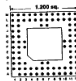
88 PINS Footprint 12008
