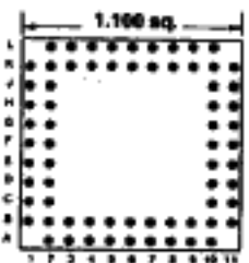
Footprint 11033
