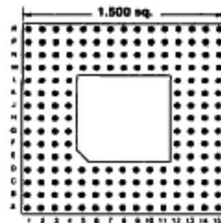
176 PINS Footprint 15013
