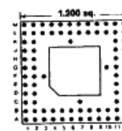
84 PINS Footprint 12010
