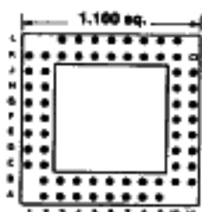
Footprint 11039
