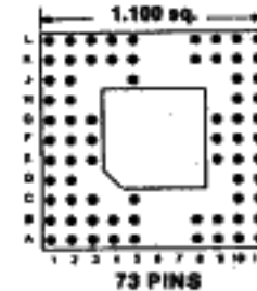
Footprint 11019
