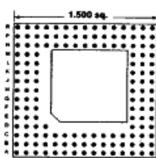
145 PINS Footprint 15023
