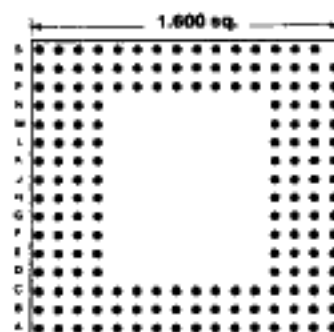
175 PINS Footprint 16008
