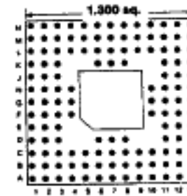
132 PINS Footprint 13006
