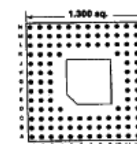
124 PINS Footprint 13008
