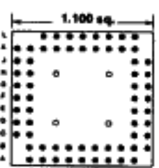
Footprint 11038
