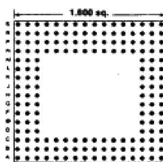
166 PINS Footprint 16004
