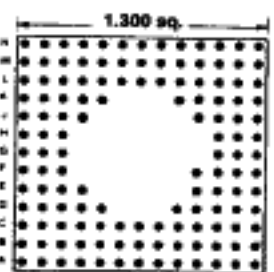
133 PINS Footprint 13052
