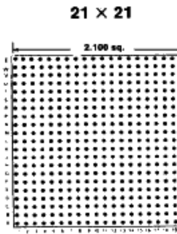
441 PINS Footprint 21001
