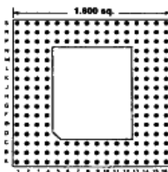
176 PINS Footprint 16006
