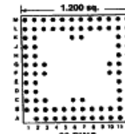
88 PINS Footprint 12009
