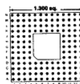
144 PINS Footprint 13002
