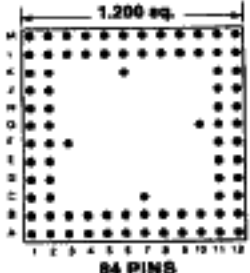
84 PINS Footprint 12011
