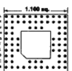
84 PINS Footprint 11009
