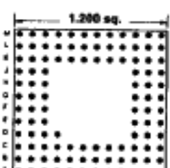
Footprint 12003
