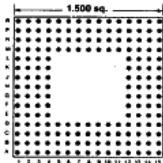
176 PINS Footprint 15014
