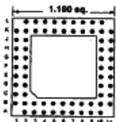
Footprint 11032
