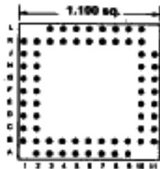
Footprint 11037
