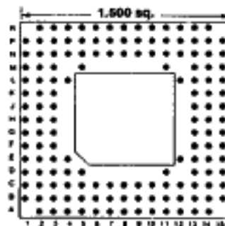
149 PINS Footprint 15018
