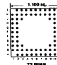
Footprint 11025
