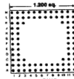
84 PINS Footprint 12013
