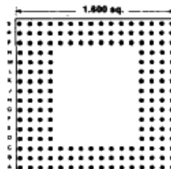
176 PINS Footprint 16007
