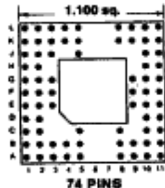
Footprint 11017
