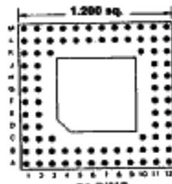
84 PINS Footprint 12012
