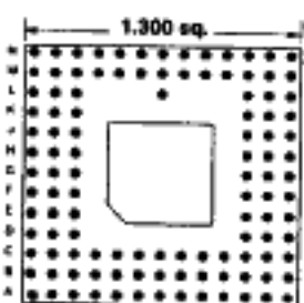
114 PINS Footprint 13051
