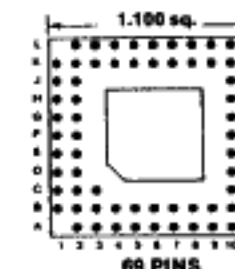
Footprint 11030
