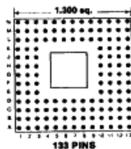
Footprint 13004
