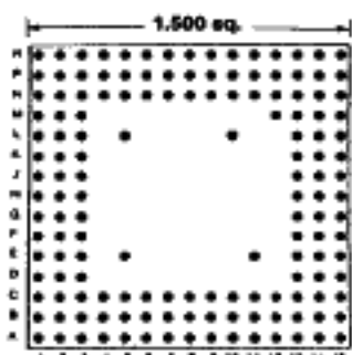
149 PINS Footprint 15020
