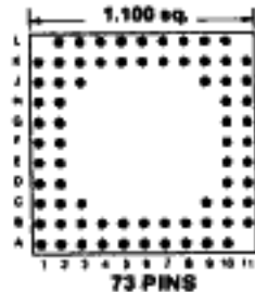
Footprint 11022
