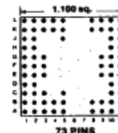
Footprint 11020
