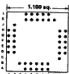
Footprint 11042
