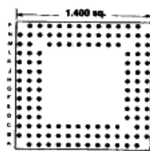
125 PINS Footprint 14021
