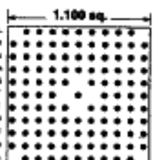
113 PINS Footprint 11004
