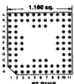
Footprint 11014
