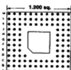
Footprint 12002
