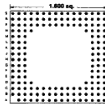
159 PINS Footprint 16009
