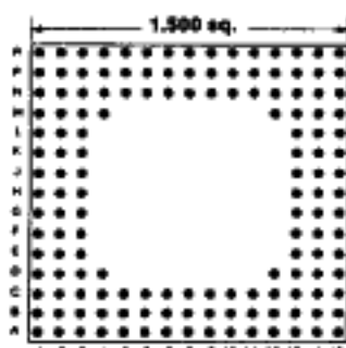
148 PINS Footprint 15022
