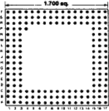
169 PINS Footprint 17002
