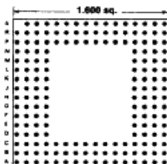
175 PINS Footprint 16003
