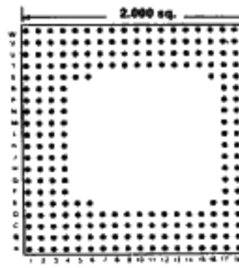
262 PINS Footprint 20003
