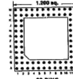
80 PINS Footprint 12014
