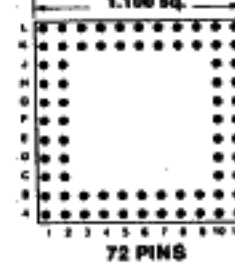
Footprint 11024
