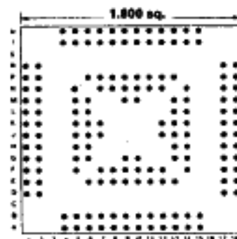
160 PINS Footprint 18011
