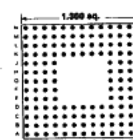
144 PINS Footprint 13003
