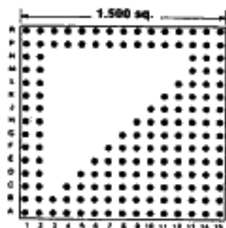
160 PINS Footprint 15015
