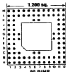
89 PINS Footprint 12006
