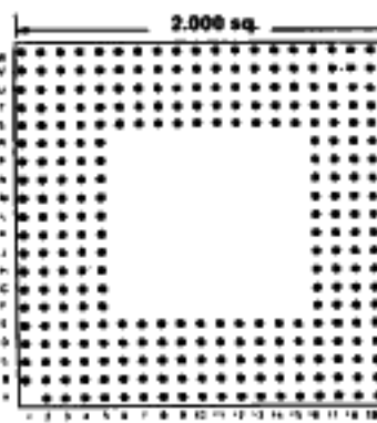
299 PINS Footprint 20002
