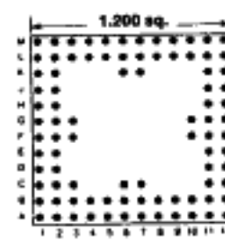
89 PINS Footprint 12007
