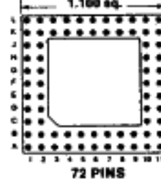
Footprint 11023
