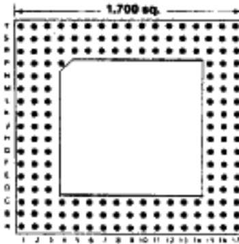
169 PINS Footprint 17010
