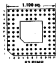
Footprint 11013
