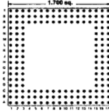
169 PINS Footprint 17011
