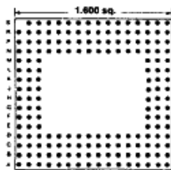
175 PINS Footprint 16005
