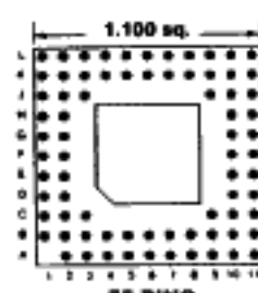
Footprint 11015
