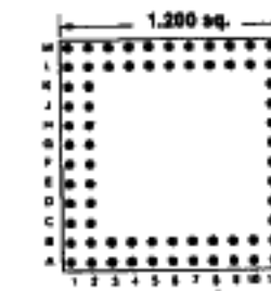
80 PINS Footprint 12015
