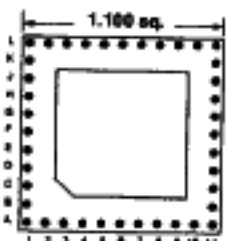
Footprint 11043
