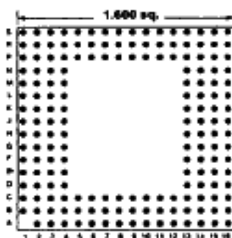
175 PINS Footprint 16010
