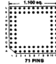
Footprint 11027
