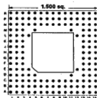
153 PINS Footprint 15016
