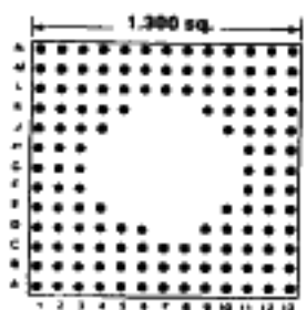
133 PINS Footprint 13046
