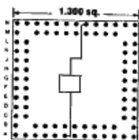
84 PINS Footprint 13056
