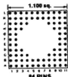
Footprint 11012
