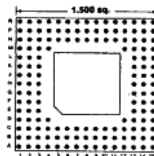
148 PINS Footprint 15021
