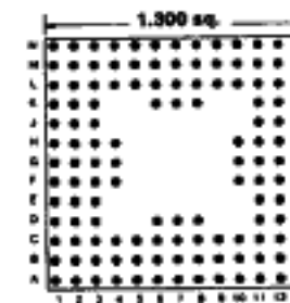
132 PINS Footprint 13007
